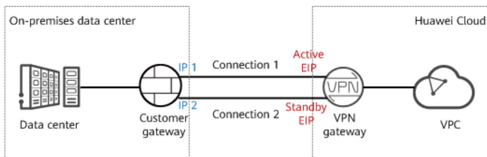
Figure 2-2 Active/Standby mode
